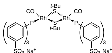
Figure 8. Schematic representation of the rhodium complex used in this study, with the two TPPTS ligands (triphenylphosphine trisulfonated-sodium salt).
