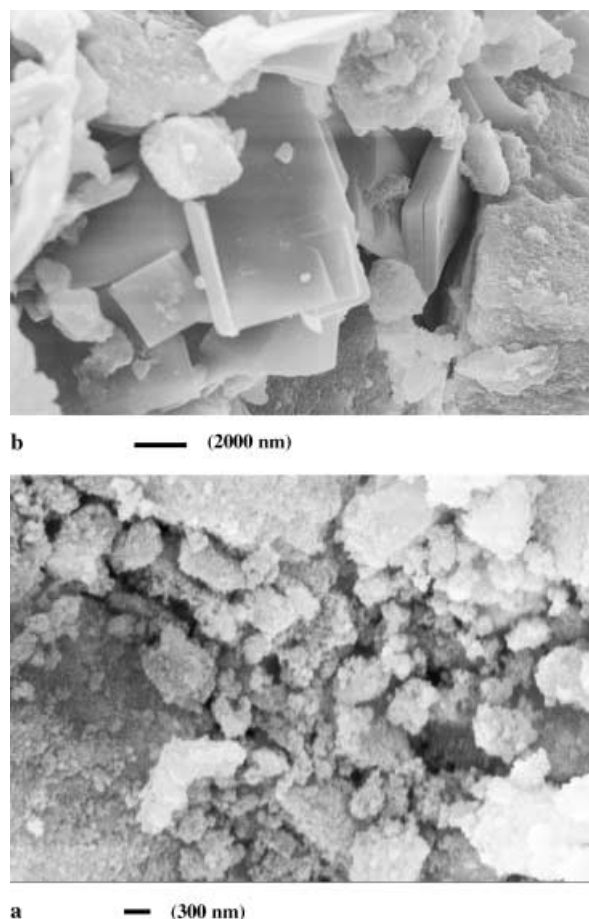
Figure 6. Scanning electron microscopy of apatitic tricalcium phosphate sample after catalytic run with a hydration rate of 20% (a) and 50% (b).
