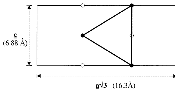
Figure 9. Representation of the calcium ions in the (001) plane.
