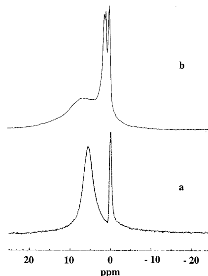
Figure 4. ^1\text{H} NMR spectra of apatitic tricalcium phosphate sample itself (a) and after a catalytic run with a hydration rate of 20% (b).
