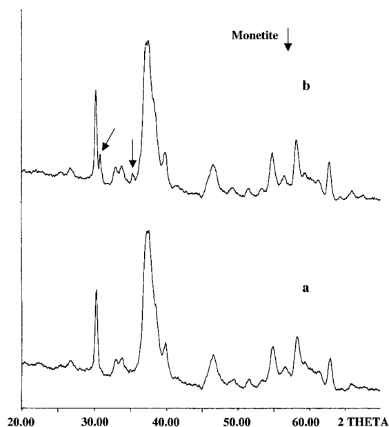
Figure 2. X-ray diffraction pattern of apatitic tricalcium phosphate samples after catalytic run carried out with a hydration rate of 20% (a), and 50% (b).
