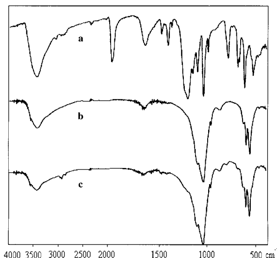
Figure 3. FTIR spectra in KBr pellets of the TPPTS rhodium complex (a), apatitic tricalcium phosphate sample itself (b), and after a catalytic run carried out with a hydration rate of 20% (c).
