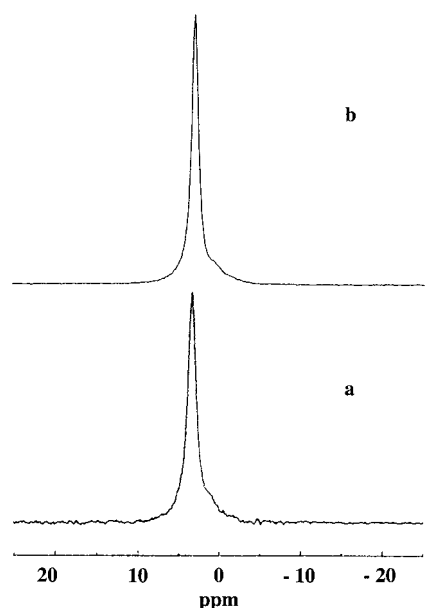
Figure 5. ^{31}\text{P} NMR spectra of apatitic tricalcium phosphate sample itself (a) and after catalytic run with a hydration rate of 20% (b).
