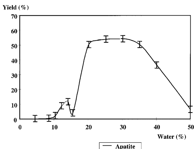
Figure 1. Yield of the hydroformylation catalytic reaction as a function of the hydration rate for apatitic tricalcium phosphate.
