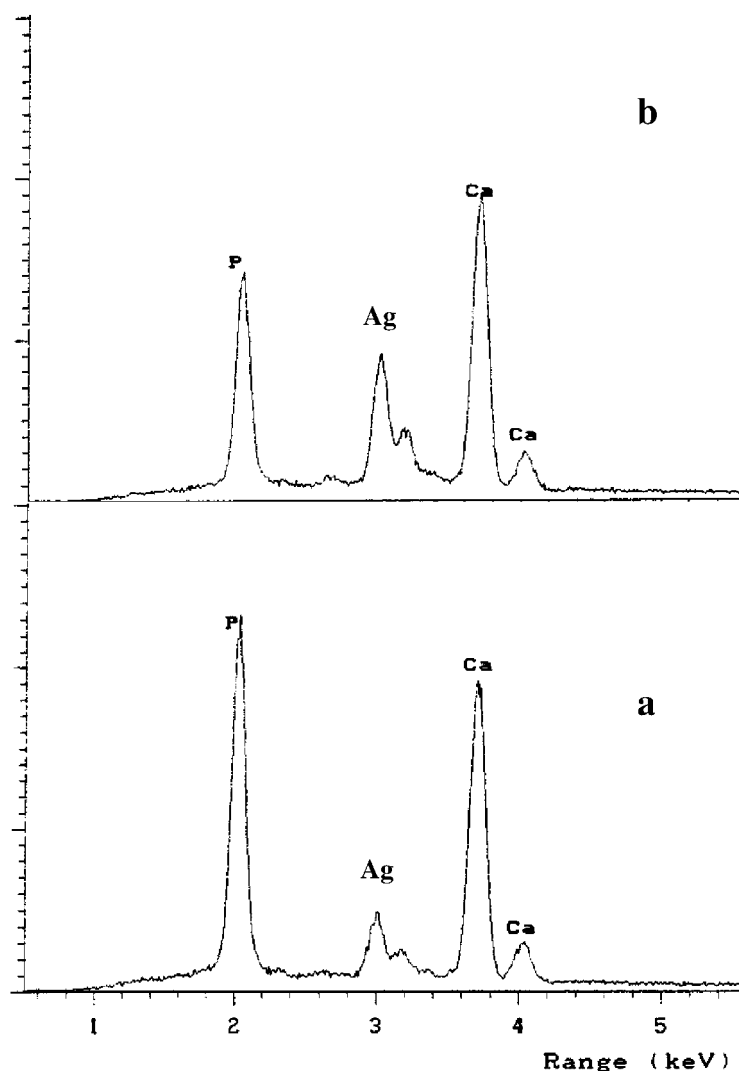
Figure 7. EDS microanalysis of apatitic tricalcium phosphate sample after catalytic run with a hydration rate of 50%: (a) plates; (b) grains.
